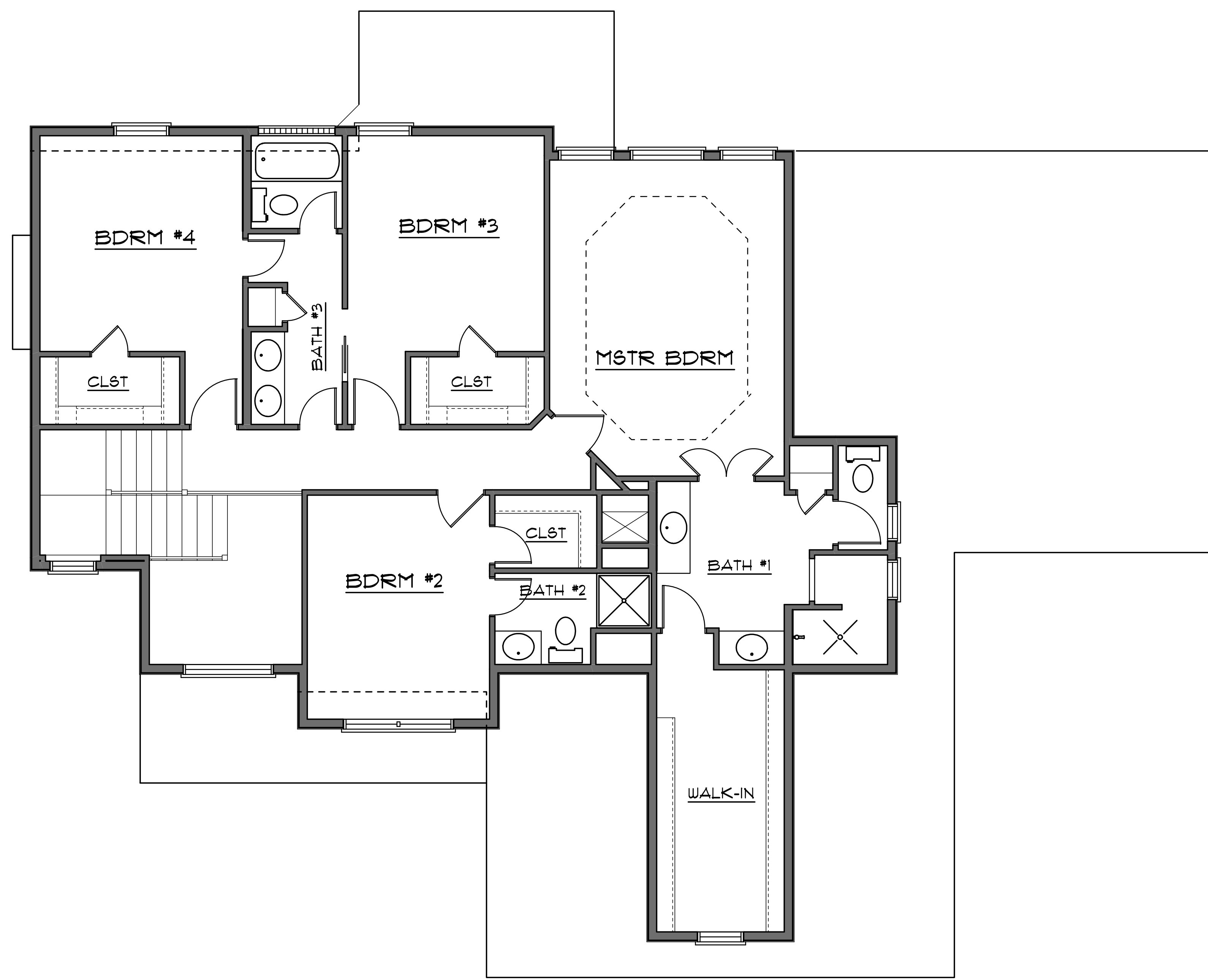
SECOND LEVEL
