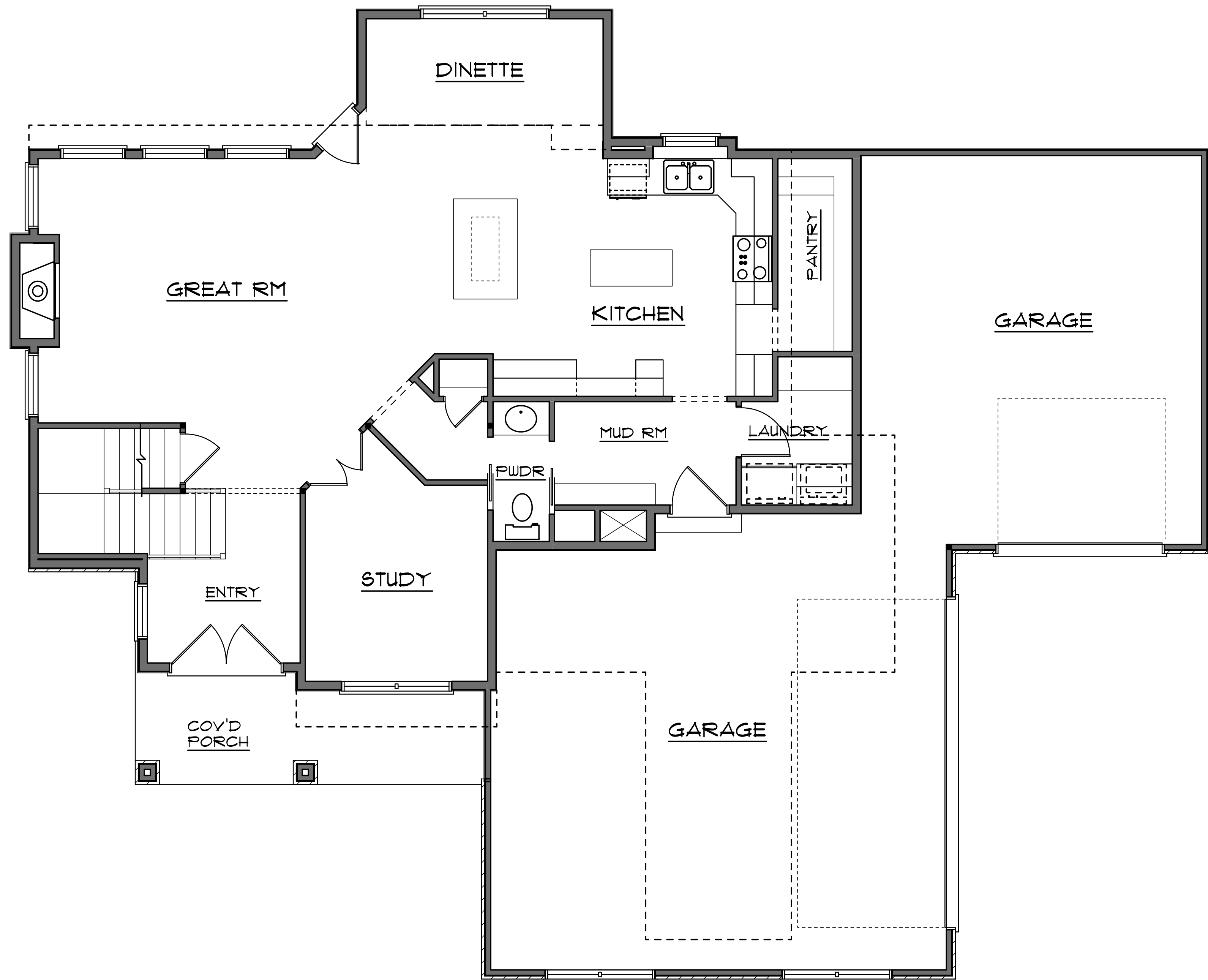
MAIN LEVEL
